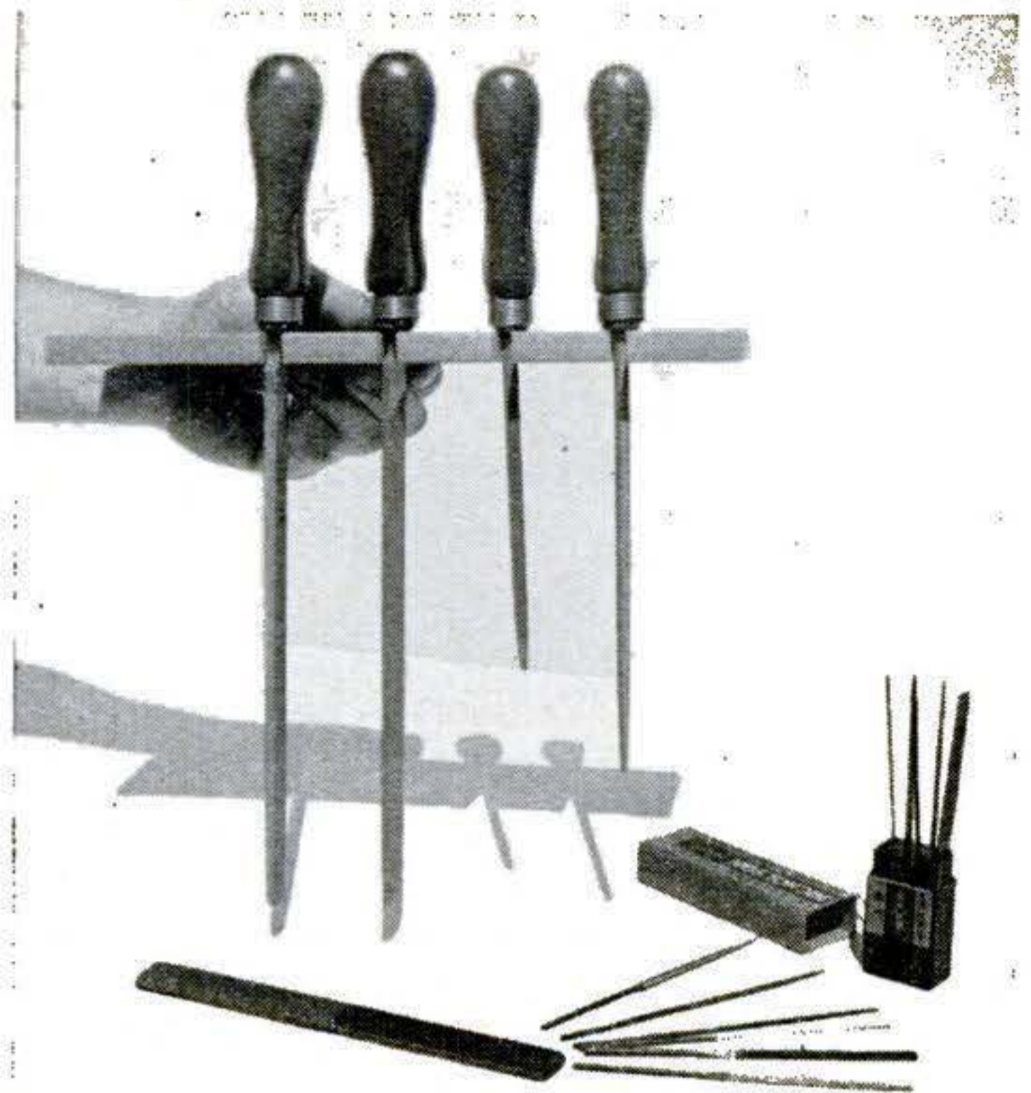
GOOD BEGINNING for a collection of files: In rack (left to right)—10" flat bastard, 10" mill bastard, 6" slim taper, 8" round bastard. On bench—8" half-round shoe rasp and set of 5½" Swiss pattern files. Notched board is fastened to wall for convenient rack.
